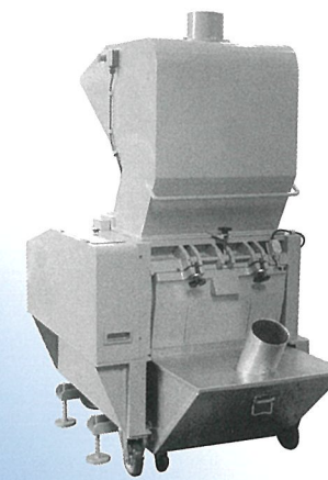
P-3060 特殊ホッパ・特殊架台・特殊受箱・集塵ホース接続タイプ Special hopper, special stand, special receptacle (with dust collector hose connected)
