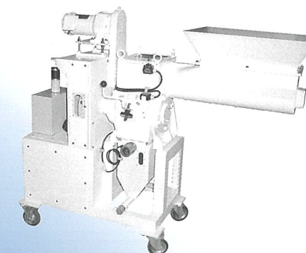
PS-180 特殊架台・特殊ホッパ・吸引空気輸送タイプ Special stand and special hopper provided with suction pneumatic transport equipment
