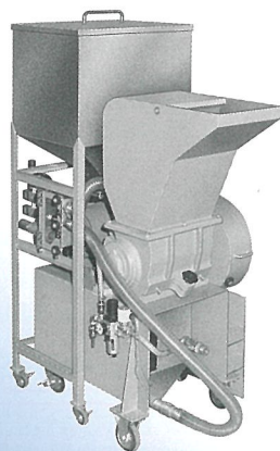
P-1328 投入シュート&L形ホッパ・原料タンク・吸引空気輸送タイプ Feed shoot and L type hopper provided with stock tank and suction pneumatic transport equipment
