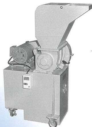
P-1328 L形ホッパ特殊高形受箱タイプ L type hopper with specially high-positioned receptacle
