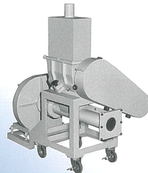
P-1328 特殊ホッパ・吸引圧送空気輸送タイプ Special hopper provided with suction pressure pneumatic transport equipment
