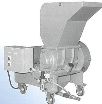
P-1328 L形ホッパブレスローダ輸送タイプ L type hopper provided with breath loader transport equipment
