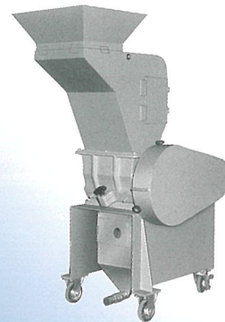
P-1328 投入シュート&特殊ホッパ・吸引空気輸送タイプ Feed shoot and special hopper provided with suction pneumatic transport equipment
