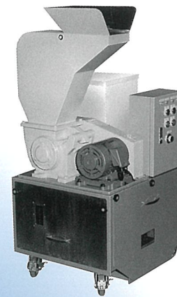
WP-1314N Z形ホッパ・原料タンク(50 l)吸引空気輸送タイプ Z type hopper and stock tank (50 l) with suction pneumatic transport equipment
