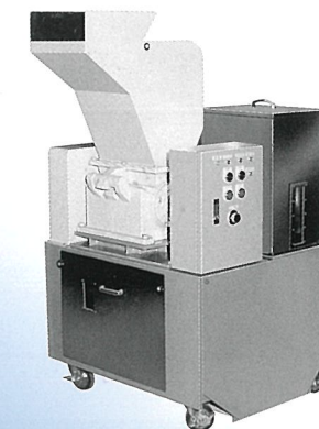
WP-1328P 特殊ホッパ・原料タンク(50 l)圧送空気輸送タイプ Special hopper and stock tank (50 l) provided with pressure pneumatic transport equipment
